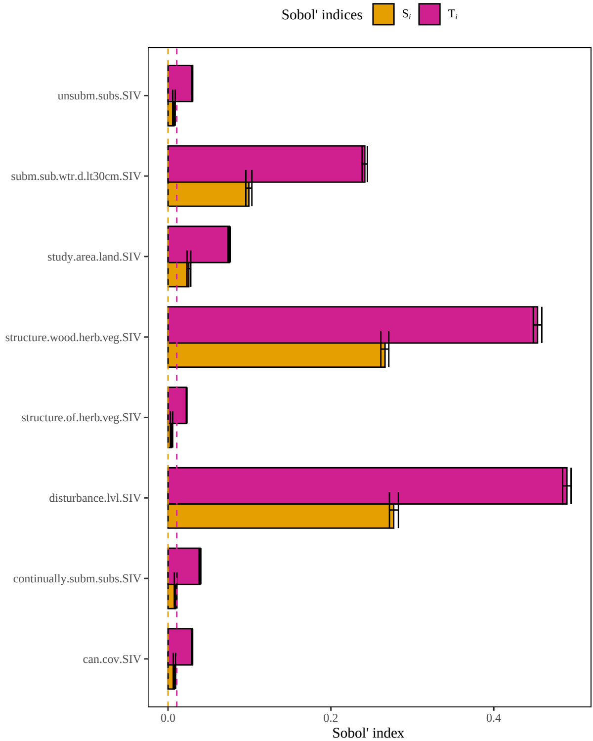
Figure 3. Results of a sensitivity analysis for the mottled duck Any model based on the original author-specified model outlined in Rorabaugh and Zwank (1983). Dashed lines represent baseline numerical approximation error for S_i and T_i ( i.e. , dummy variables).
