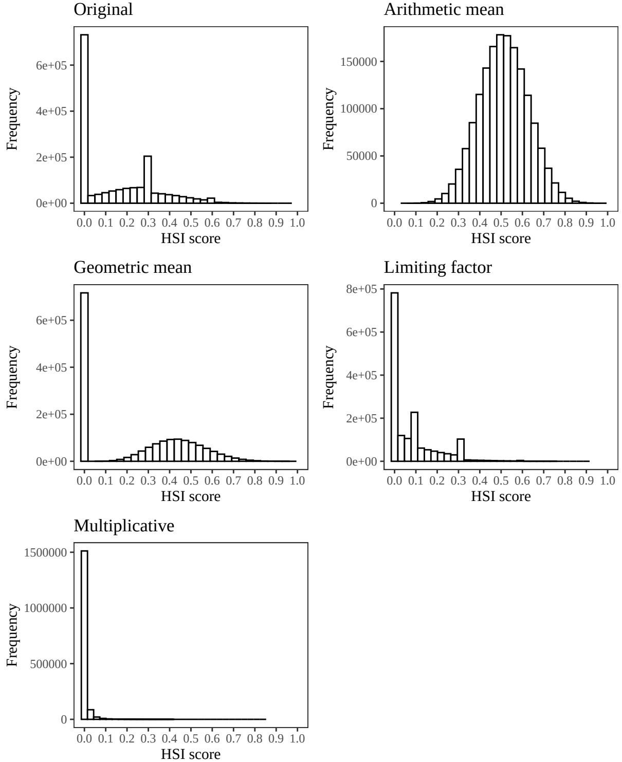
Figure 2. Empirical distributions of HSI scores for the mottled duck Any model using the original author-specified model equation from Rorabaugh and Zwank (1983), and an arithmetic mean, geometric mean, limiting factor, and multiplicative structure incorporating all SIV variables. Note differences in the y axis.
